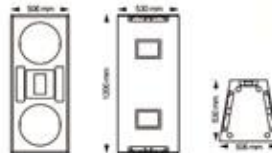
DW25 双15寸全频音箱 DUAL 15" STAGE SPEAKER
