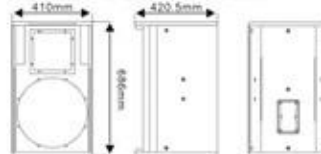
MC15 单15寸全频 SINGLE 15" ENTERTAINMENT SPEAKER
