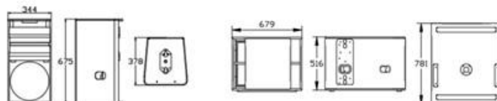
S1210 单12寸线阵 SINGLE 12" LINE ARRAY SPEAKER
